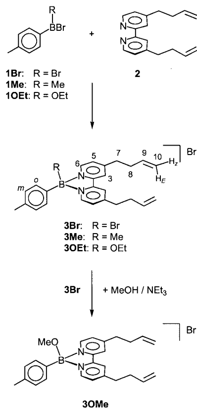
Scheme 2. Synthesis of the 2,2'-bipyridylboronium bromides 3Br , 3Me , 3OEt and 3OMe .
